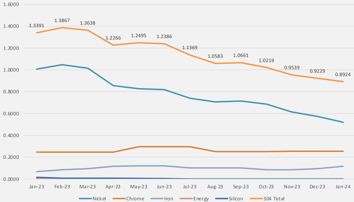
304/304L Surcharges
