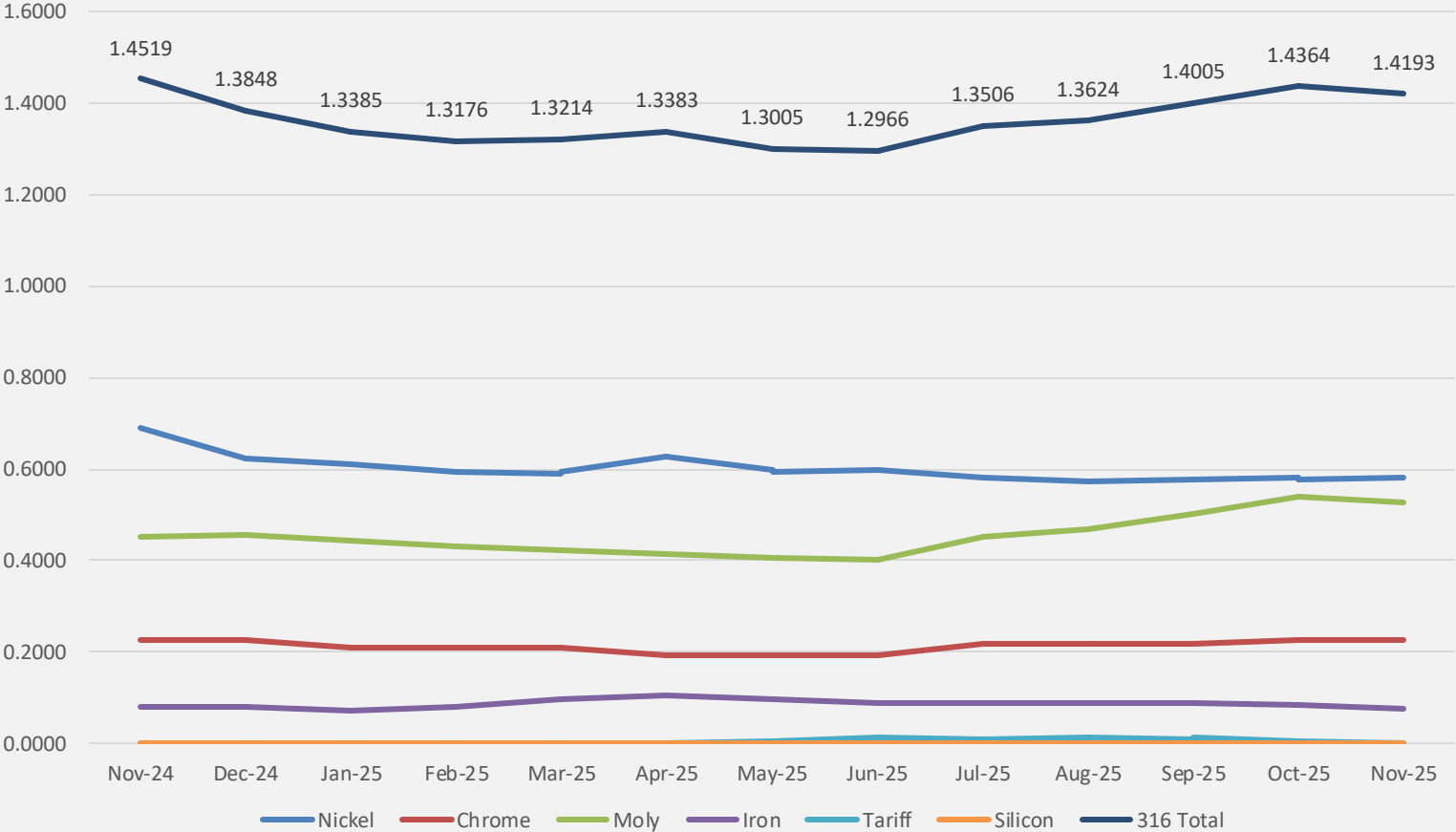
316/316L Surcharges
